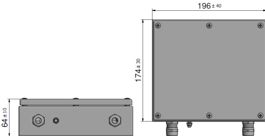
Fig.4. External view– dimensions
