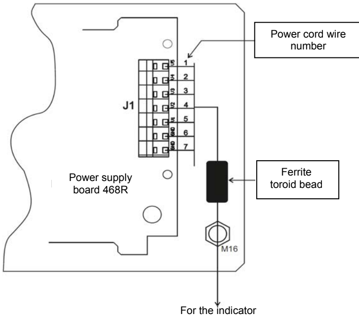
Fig.7. Connection method of the intrinsically safe cable
